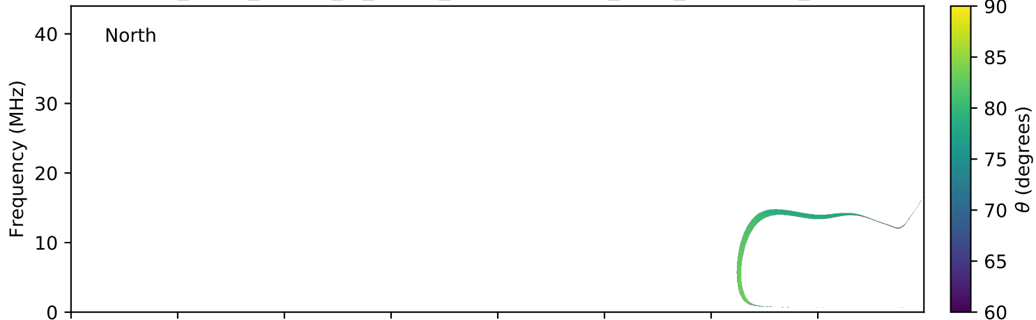
expres_earth_jupiter_io_jrm09_lossc-wid1deg_3kev_20111126_v01.cdf
