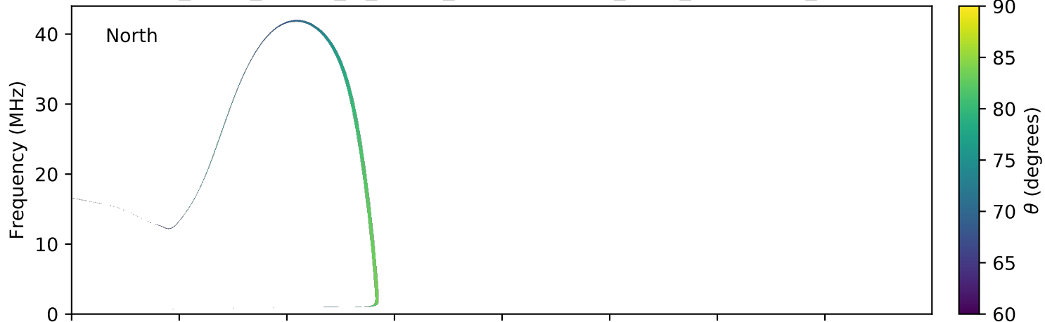
expres_earth_jupiter_io_jrm09_lossc-wid1deg_3kev_20111122_v01.cdf
