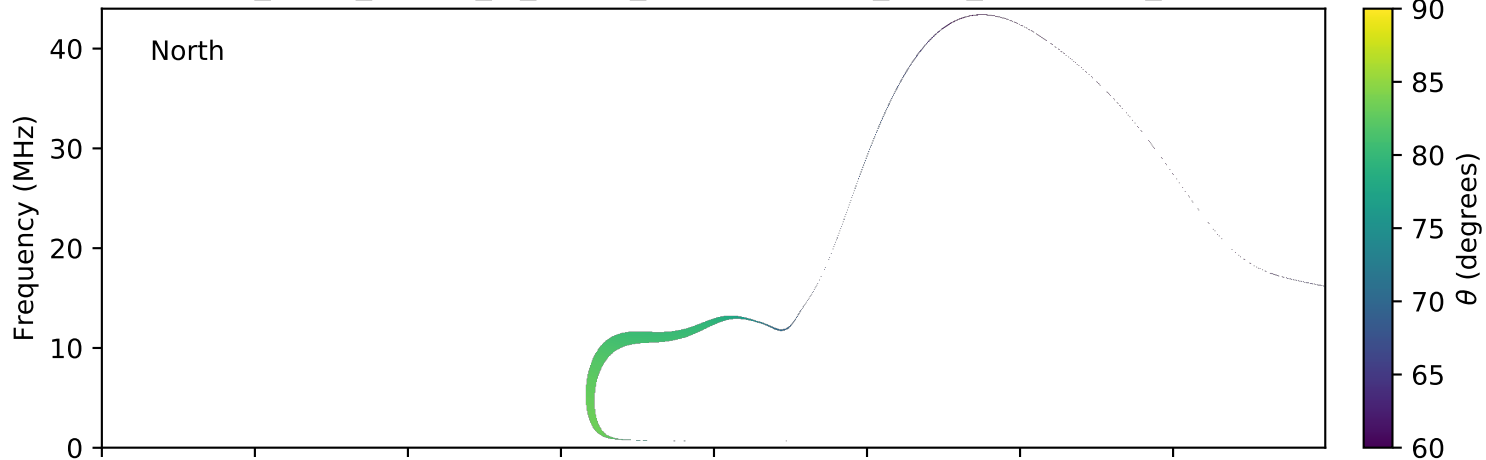
expres_earth_jupiter_io_jrm09_lossc-wid1deg_3kev_20111114_v01.cdf
