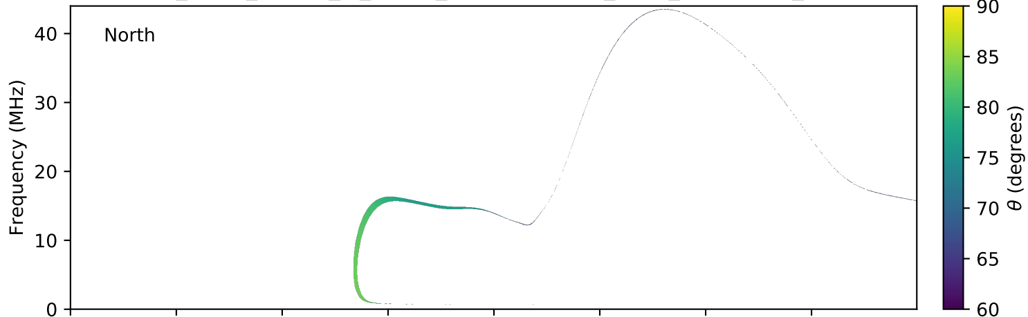
expres_earth_jupiter_io_jrm09_lossc-wid1deg_3kev_20111107_v01.cdf
