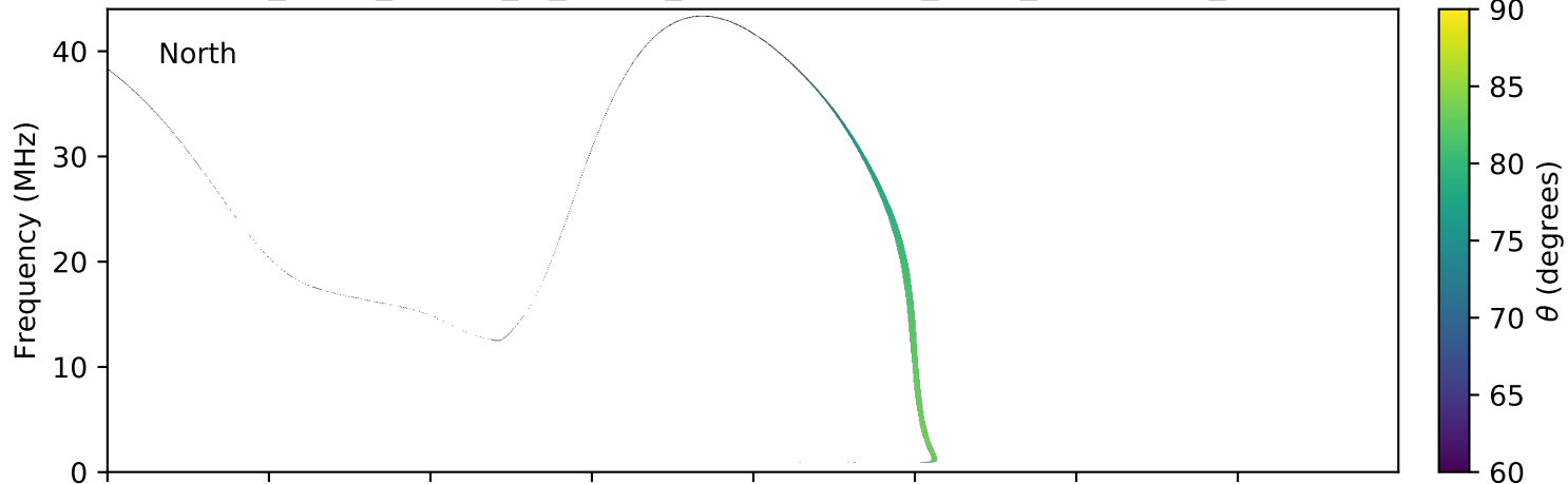
expres_earth_jupiter_io_jrm09_lossc-wid1deg_3kev_20111104_v01.cdf
