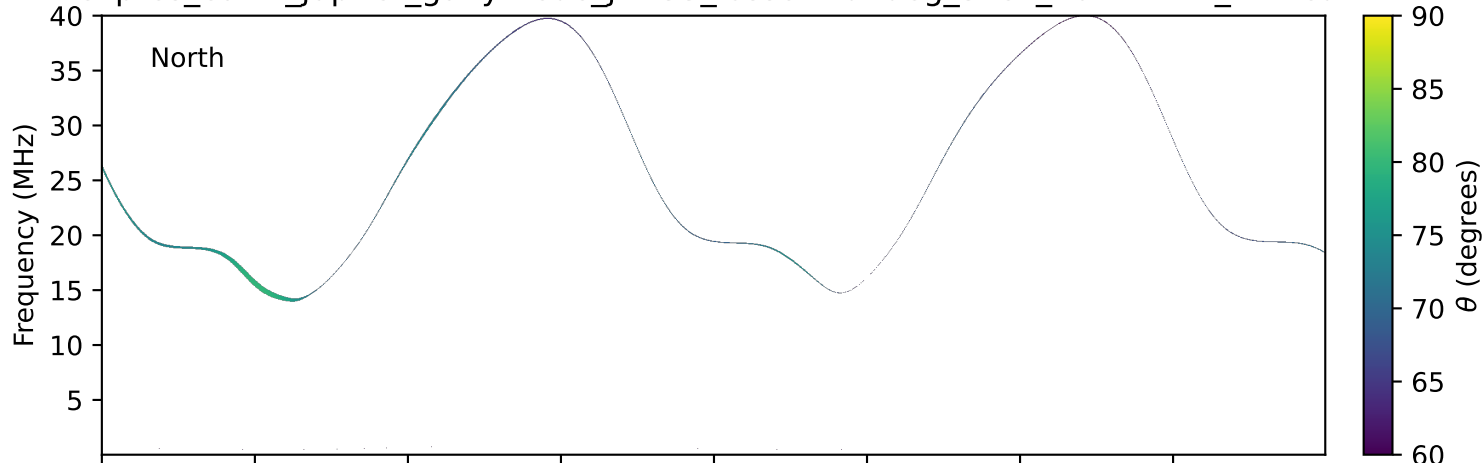
expres_earth_jupiter_ganymede_jrm33_lossc-wid1deg_3kev_20111121_v11.cdf
