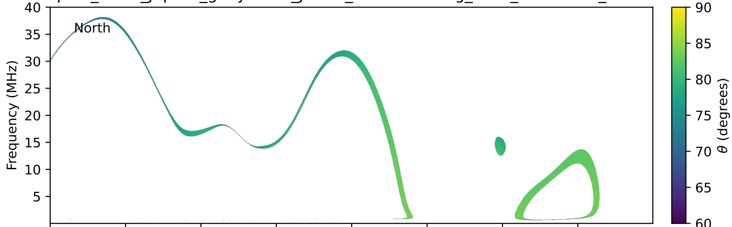
expres_earth_jupiter_ganymede_jrm33_lossc-wid1deg_3kev_20111116_v11.cdf
