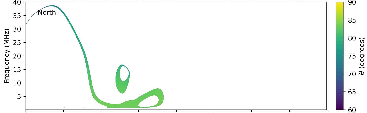
expres_earth_jupiter_europa_jrm33_lossc-wid1deg_3kev_20111116_v11.cdf
