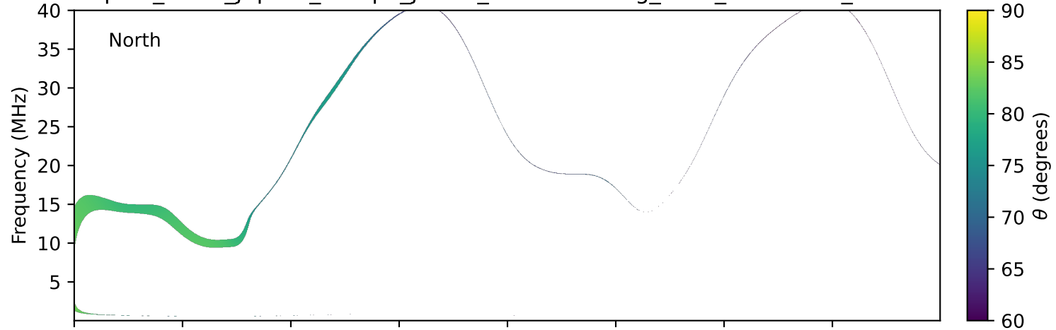
expres_earth_jupiter_europa_jrm33_lossc-wid1deg_3kev_20111104_v11.cdf
