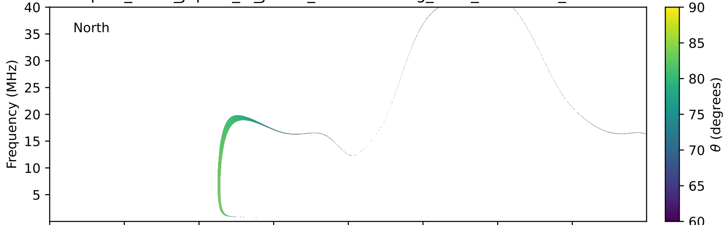
expres_earth_jupiter_io_jrm33_lossc-wid1deg_3kev_20111031_v11.cdf
