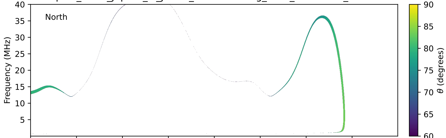
expres_earth_jupiter_io_jrm33_lossc-wid1deg_3kev_20111026_v11.cdf
