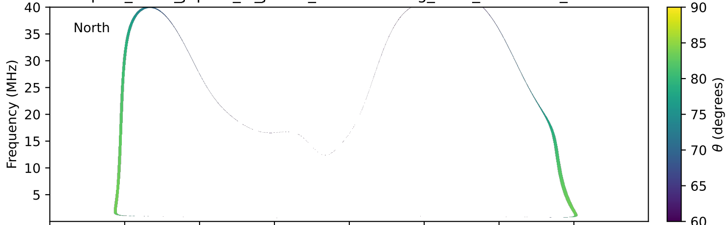
expres_earth_jupiter_io_jrm33_lossc-wid1deg_3kev_20111010_v11.cdf
