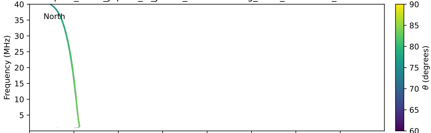
expres_earth_jupiter_io_jrm33_lossc-wid1deg_3kev_20111009_v11.cdf
