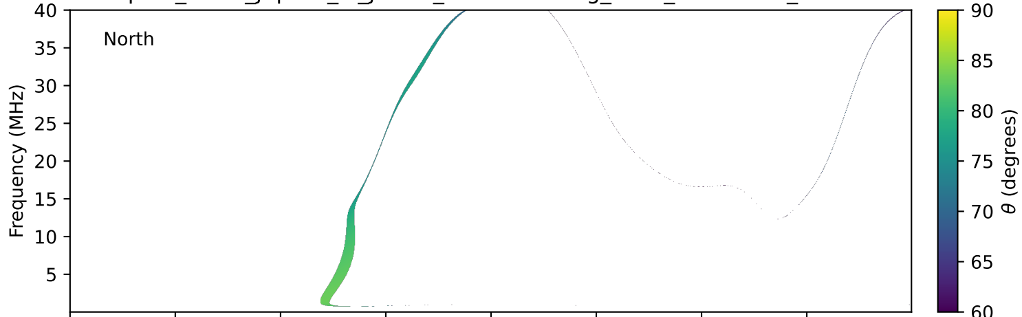
expres_earth_jupiter_io_jrm33_lossc-wid1deg_3kev_20111008_v11.cdf
