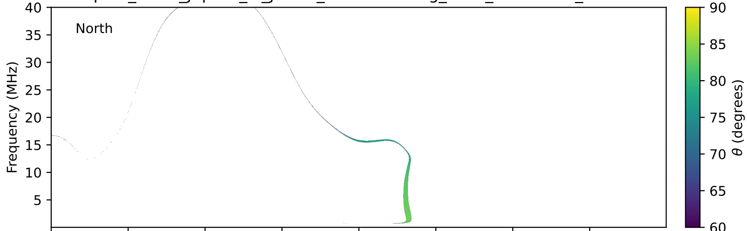
expres_earth_jupiter_io_jrm33_lossc-wid1deg_3kev_20111005_v11.cdf
