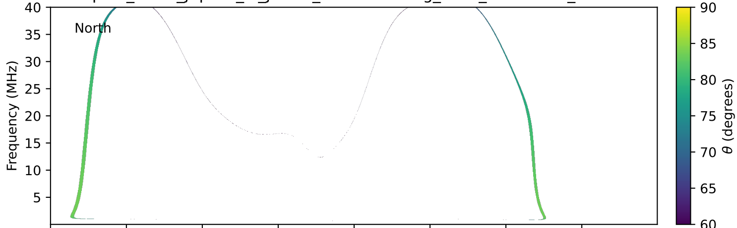
expres_earth_jupiter_io_jrm33_lossc-wid1deg_3kev_20111003_v11.cdf
