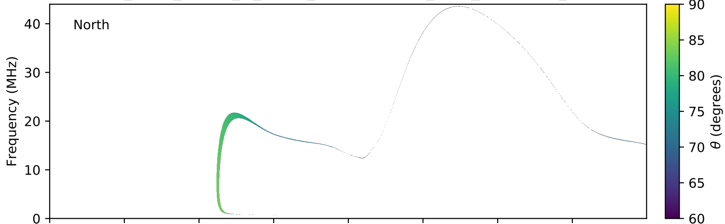
expres_earth_jupiter_io_jrm09_lossc-wid1deg_3kev_20111031_v01.cdf
