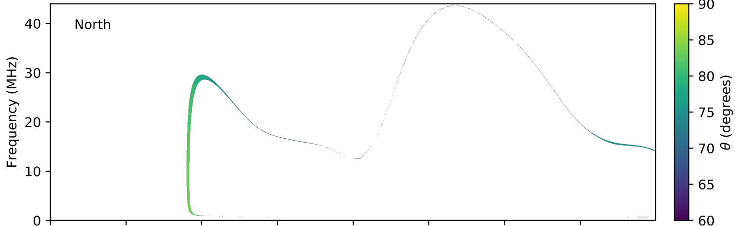
expres_earth_jupiter_io_jrm09_lossc-wid1deg_3kev_20111024_v01.cdf
