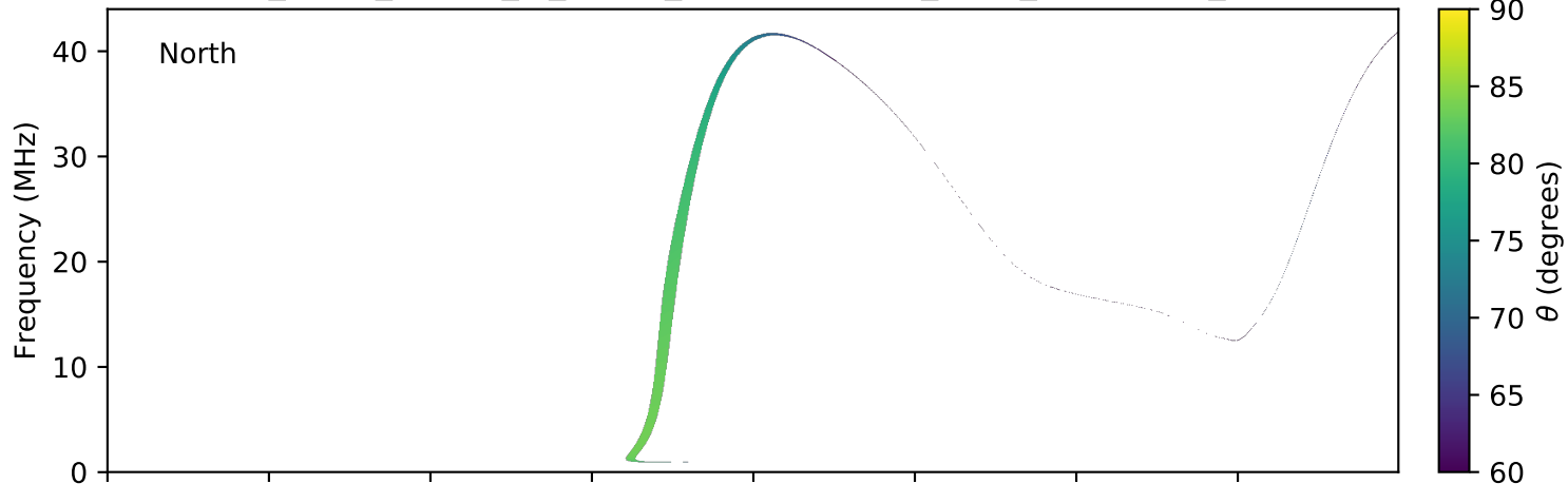
expres_earth_jupiter_io_jrm09_lossc-wid1deg_3kev_20111015_v01.cdf
