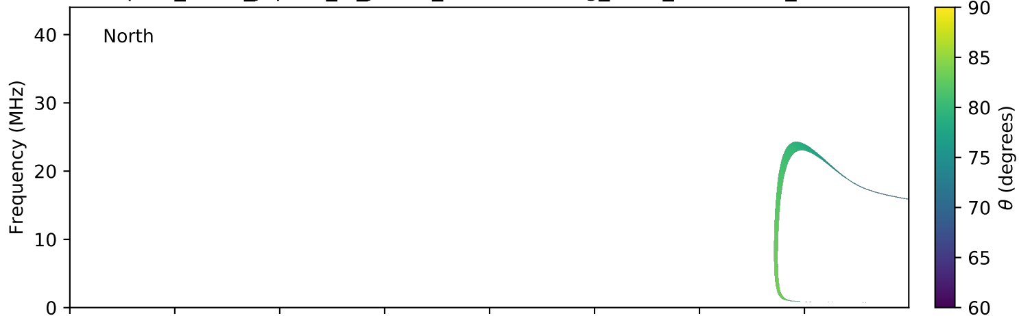
expres_earth_jupiter_io_jrm09_lossc-wid1deg_3kev_20111011_v01.cdf
