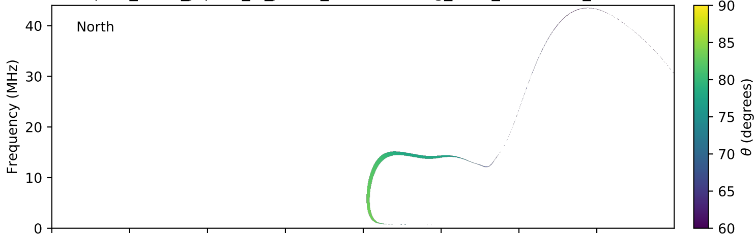
expres_earth_jupiter_io_jrm09_lossc-wid1deg_3kev_20111006_v01.cdf
