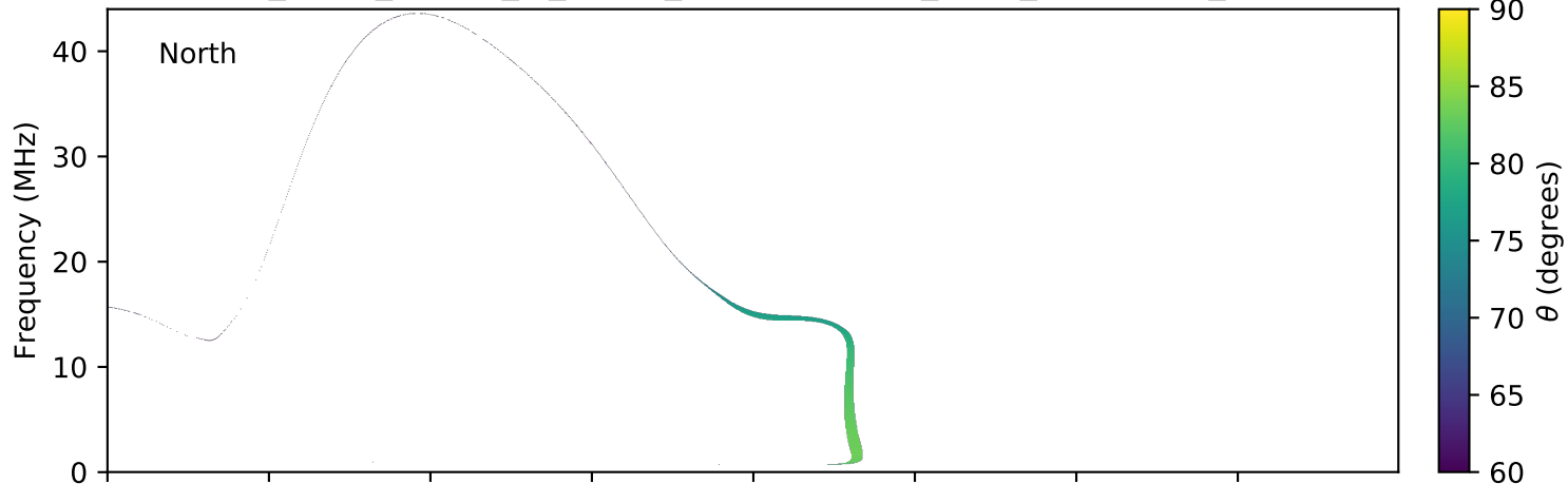
expres_earth_jupiter_io_jrm09_lossc-wid1deg_3kev_20111005_v01.cdf
