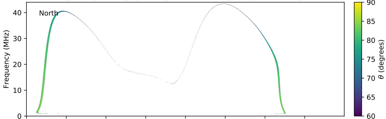
expres_earth_jupiter_io_jrm09_lossc-wid1deg_3kev_20111003_v01.cdf
