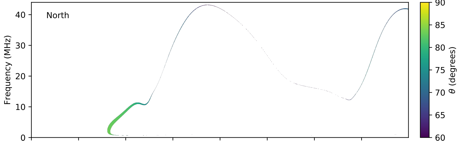
expres_earth_jupiter_io_jrm09_lossc-wid1deg_3kev_20111001_v01.cdf
