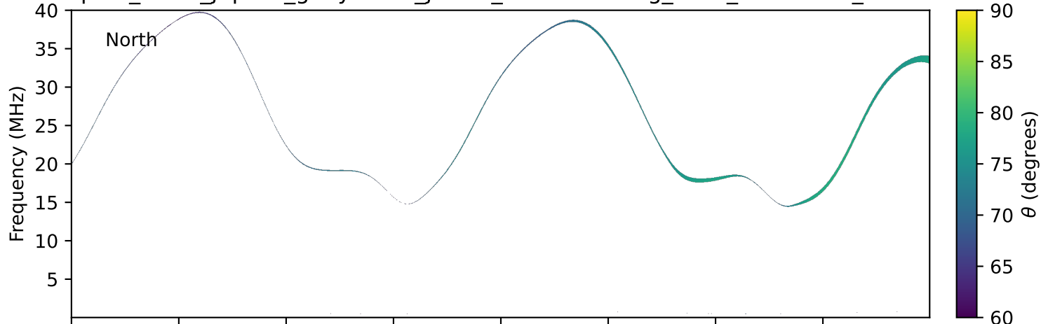
expres_earth_jupiter_ganymede_jrm33_lossc-wid1deg_3kev_20111025_v11.cdf
