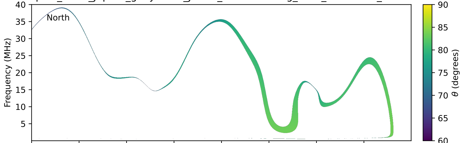
expres_earth_jupiter_ganymede_jrm33_lossc-wid1deg_3kev_20111004_v11.cdf
