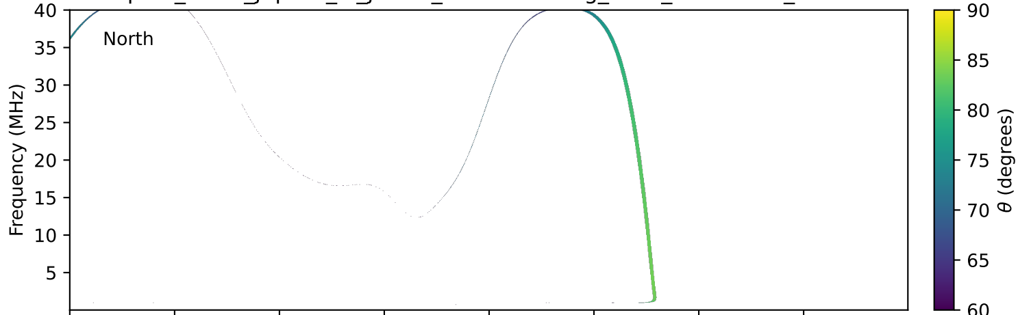
expres_earth_jupiter_io_jrm33_lossc-wid1deg_3kev_20110919_v11.cdf
