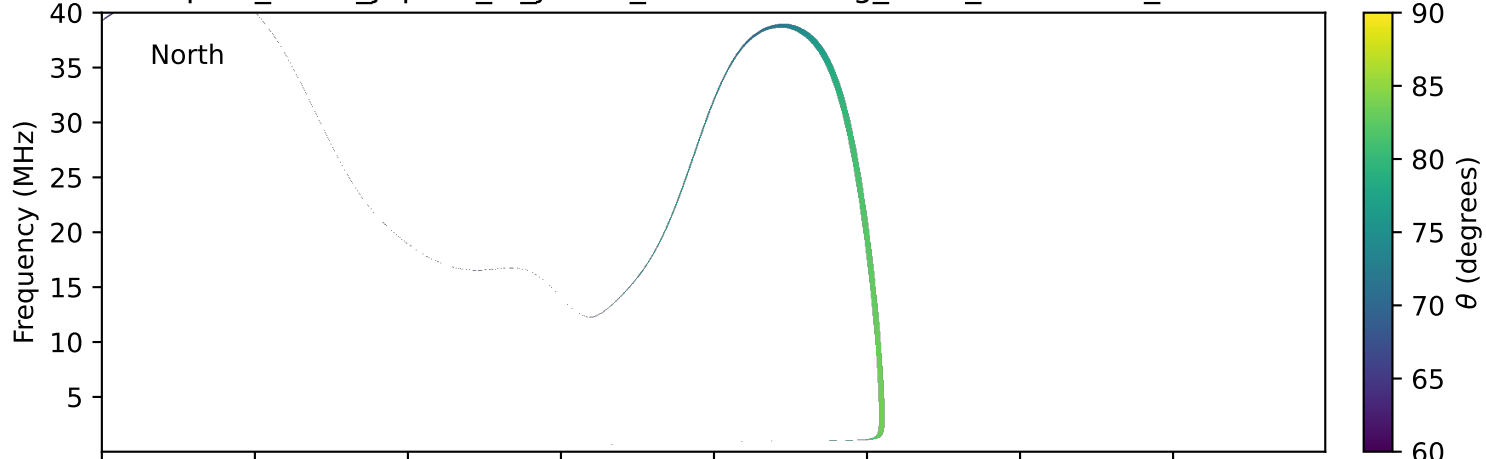
expres_earth_jupiter_io_jrm33_lossc-wid1deg_3kev_20110912_v11.cdf
