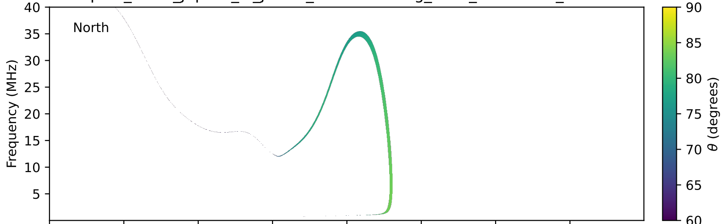
expres_earth_jupiter_io_jrm33_lossc-wid1deg_3kev_20110905_v11.cdf
