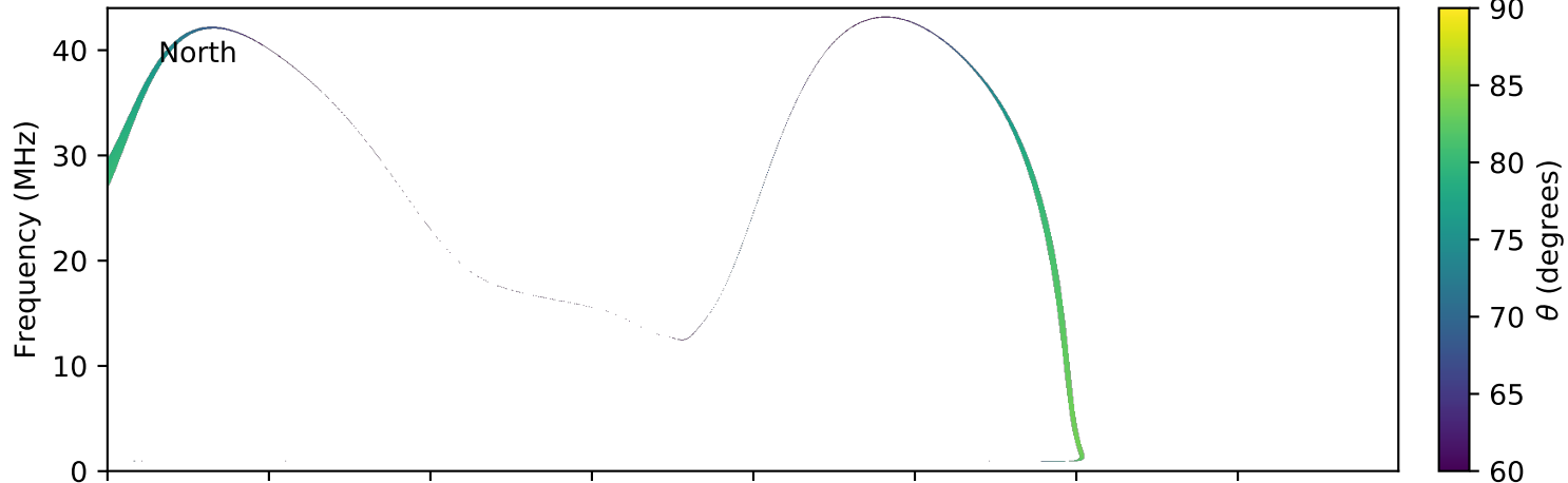
expres_earth_jupiter_io_jrm09_lossc-wid1deg_3kev_20110926_v01.cdf
