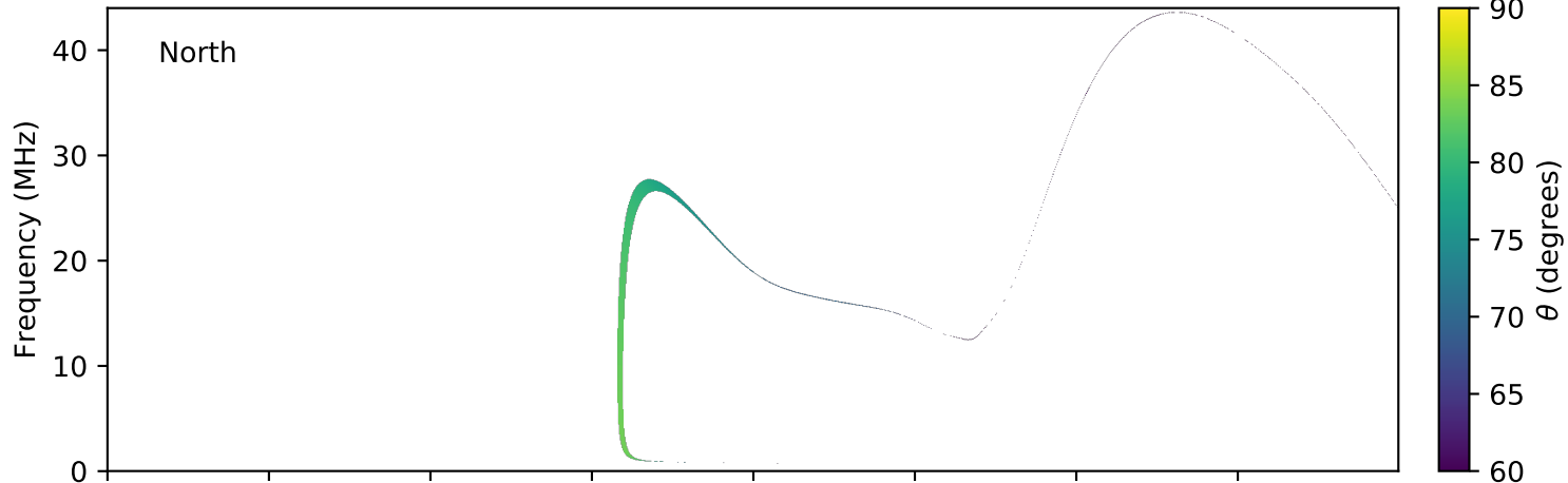
expres_earth_jupiter_io_jrm09_lossc-wid1deg_3kev_20110922_v01.cdf
