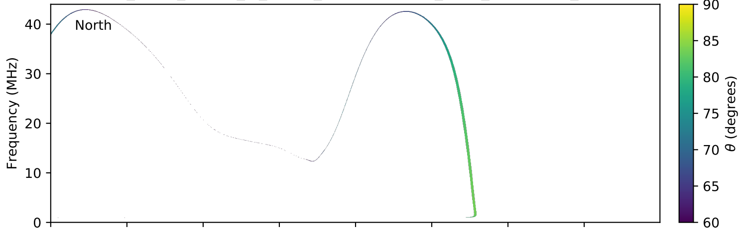
expres_earth_jupiter_io_jrm09_lossc-wid1deg_3kev_20110919_v01.cdf
