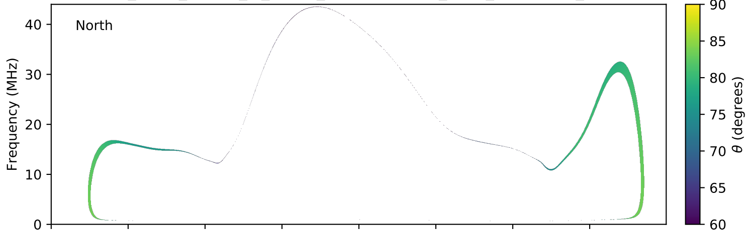
expres_earth_jupiter_io_jrm09_lossc-wid1deg_3kev_20110917_v01.cdf
