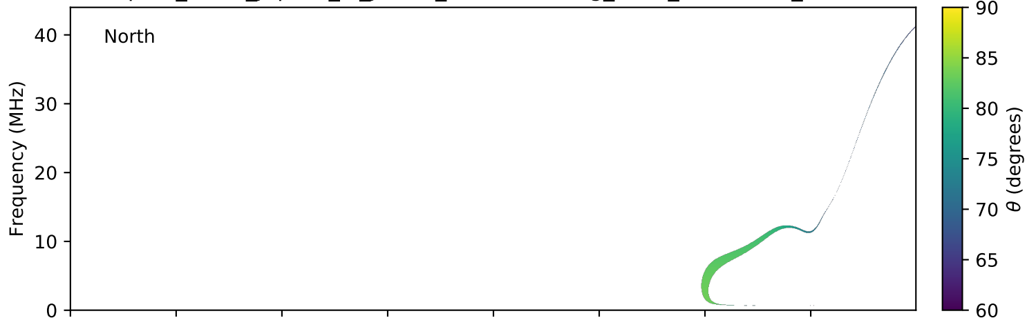
expres_earth_jupiter_io_jrm09_lossc-wid1deg_3kev_20110911_v01.cdf
