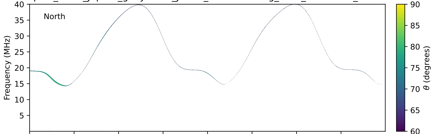
expres_earth_jupiter_ganymede_jrm33_lossc-wid1deg_3kev_20110925_v11.cdf
