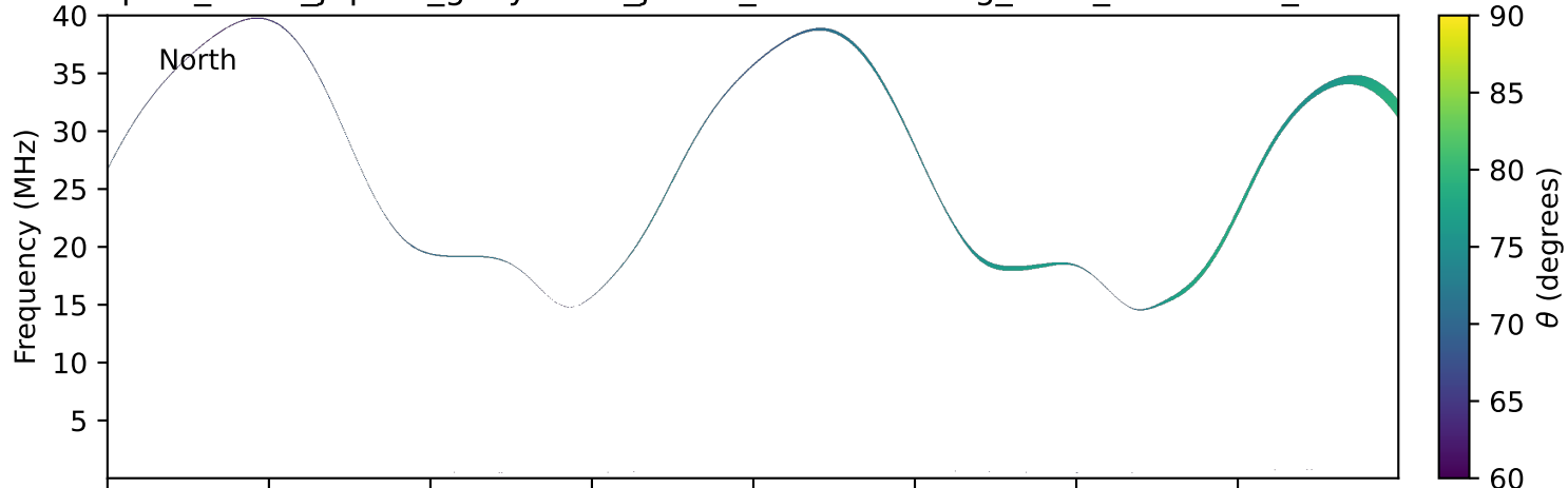
expres_earth_jupiter_ganymede_jrm33_lossc-wid1deg_3kev_20110905_v11.cdf
