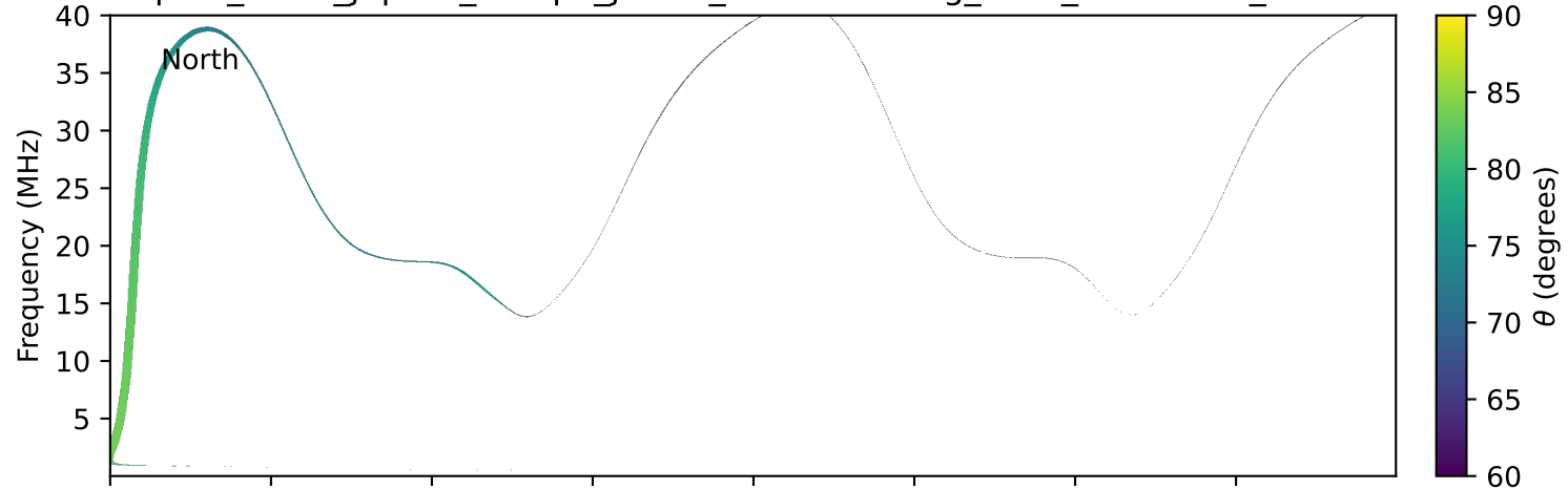
expres_earth_jupiter_europa_jrm33_lossc-wid1deg_3kev_20110919_v11.cdf
