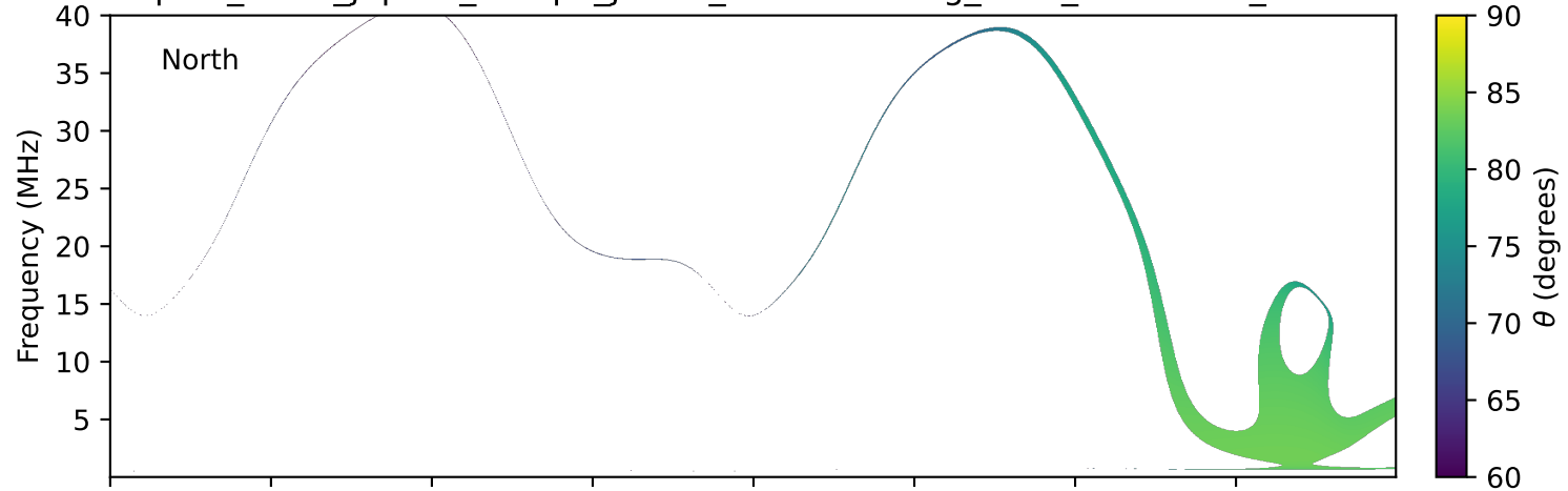
expres_earth_jupiter_europa_jrm33_lossc-wid1deg_3kev_20110909_v11.cdf
