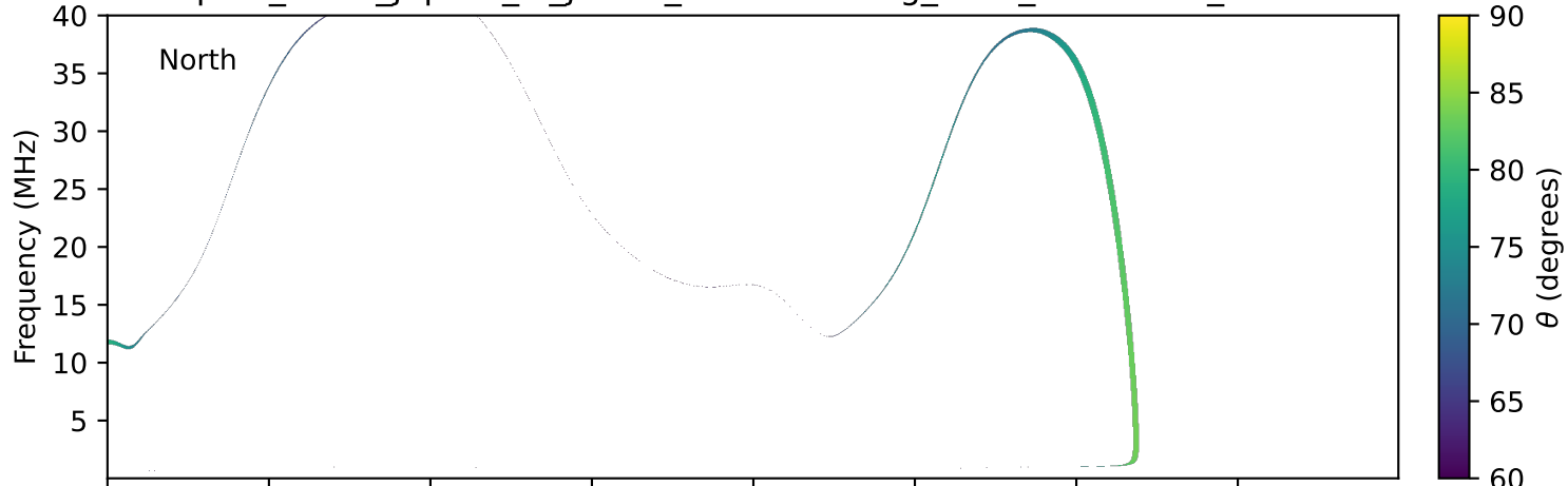
expres_earth_jupiter_io_jrm33_lossc-wid1deg_3kev_20110811_v11.cdf
