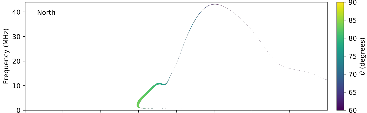
expres_earth_jupiter_io_jrm09_lossc-wid1deg_3kev_20110830_v01.cdf
