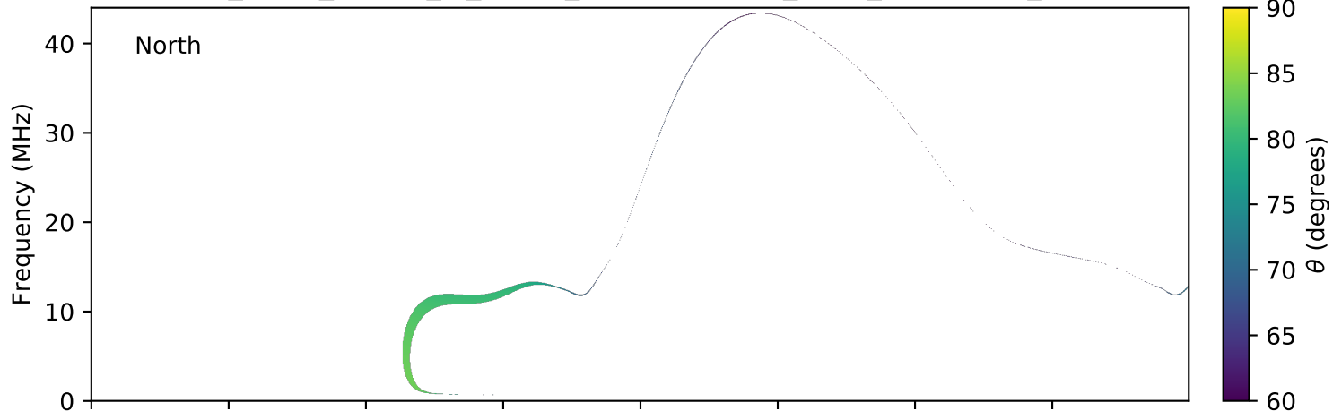
expres_earth_jupiter_io_jrm09_lossc-wid1deg_3kev_20110823_v01.cdf
