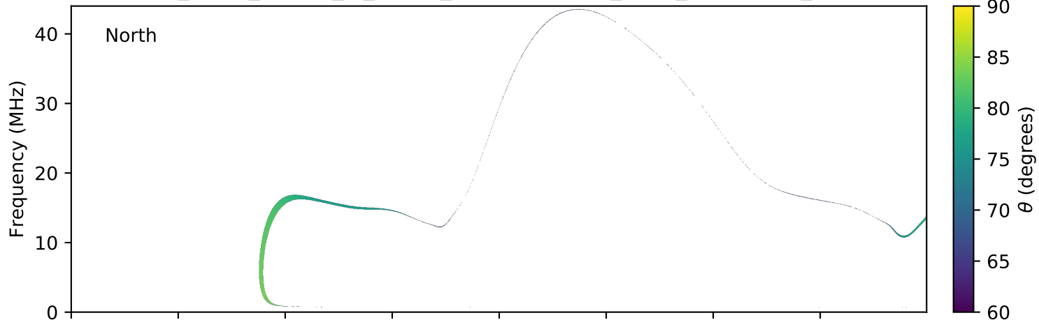
expres_earth_jupiter_io_jrm09_lossc-wid1deg_3kev_20110816_v01.cdf
