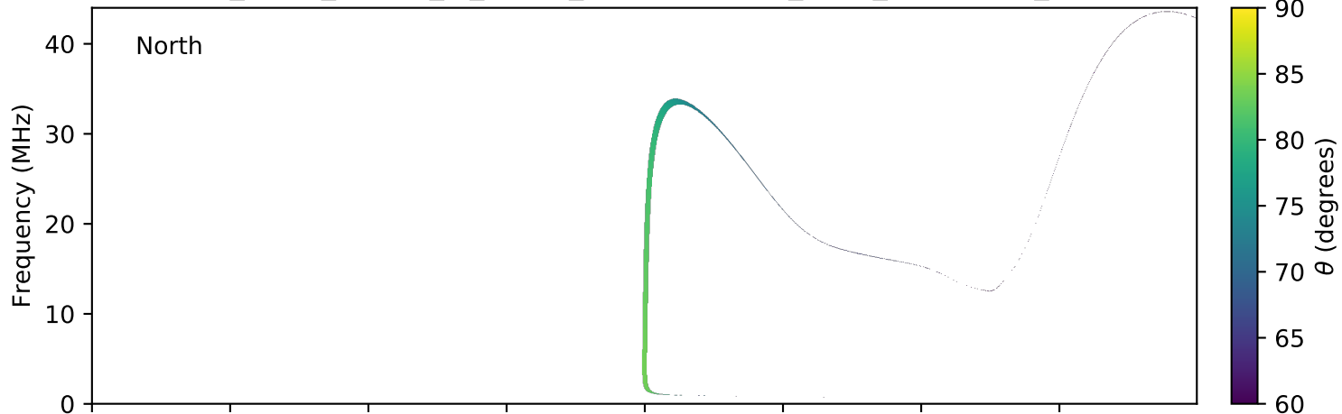
expres_earth_jupiter_io_jrm09_lossc-wid1deg_3kev_20110814_v01.cdf
