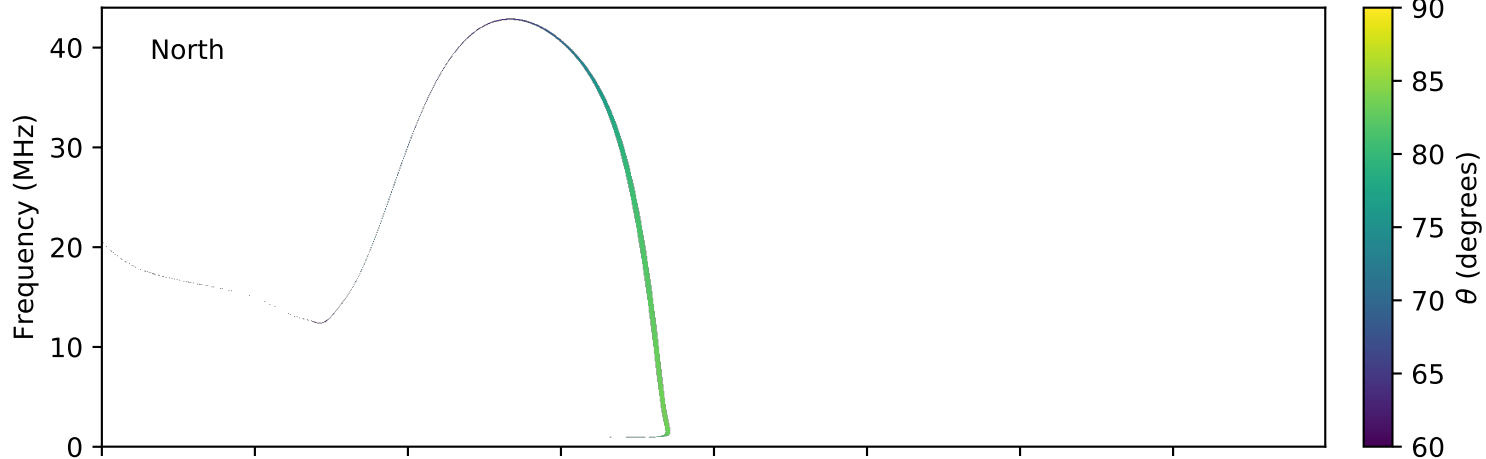
expres_earth_jupiter_io_jrm09_lossc-wid1deg_3kev_20110806_v01.cdf
