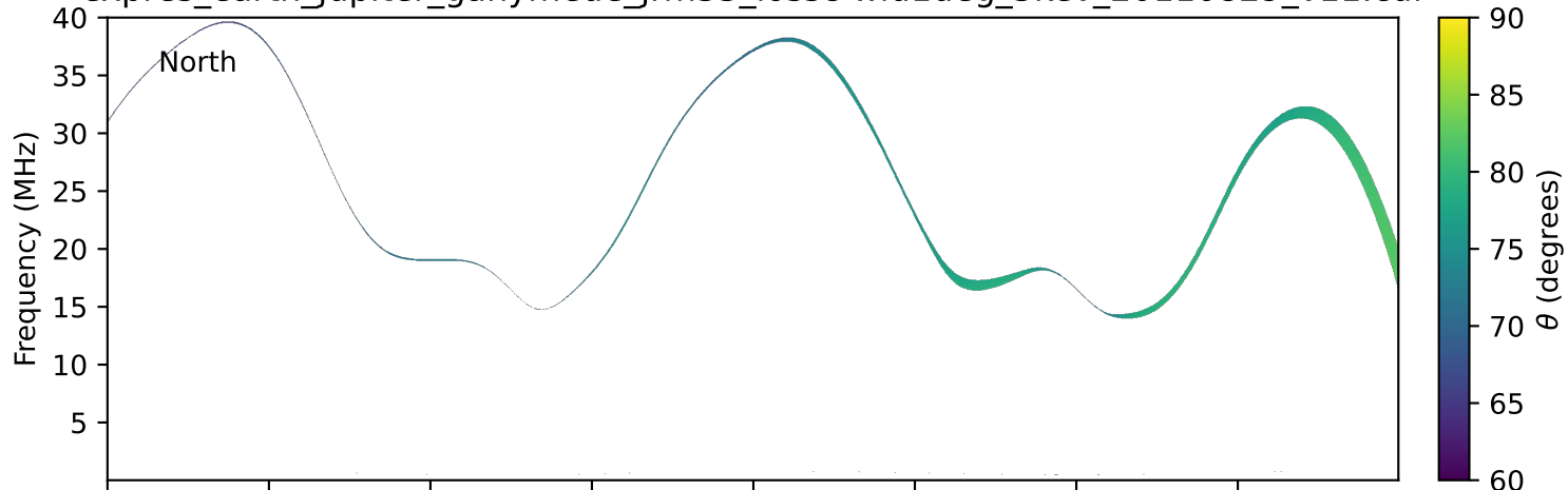
expres_earth_jupiter_ganymede_jrm33_lossc-wid1deg_3kev_20110829_v11.cdf
