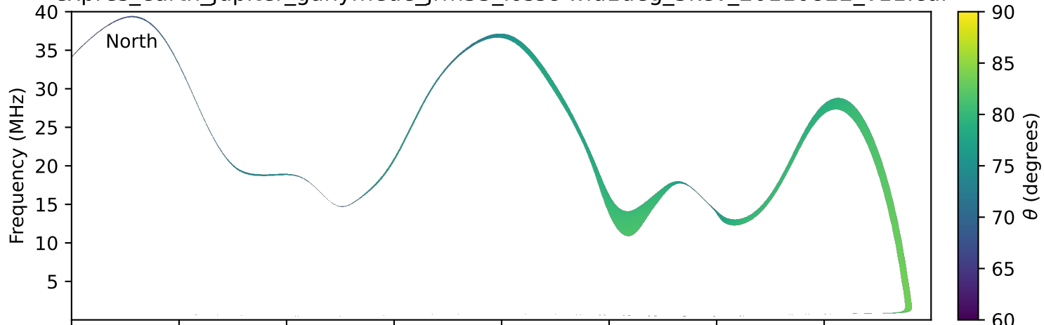
expres_earth_jupiter_ganymede_jrm33_lossc-wid1deg_3kev_20110822_v11.cdf
