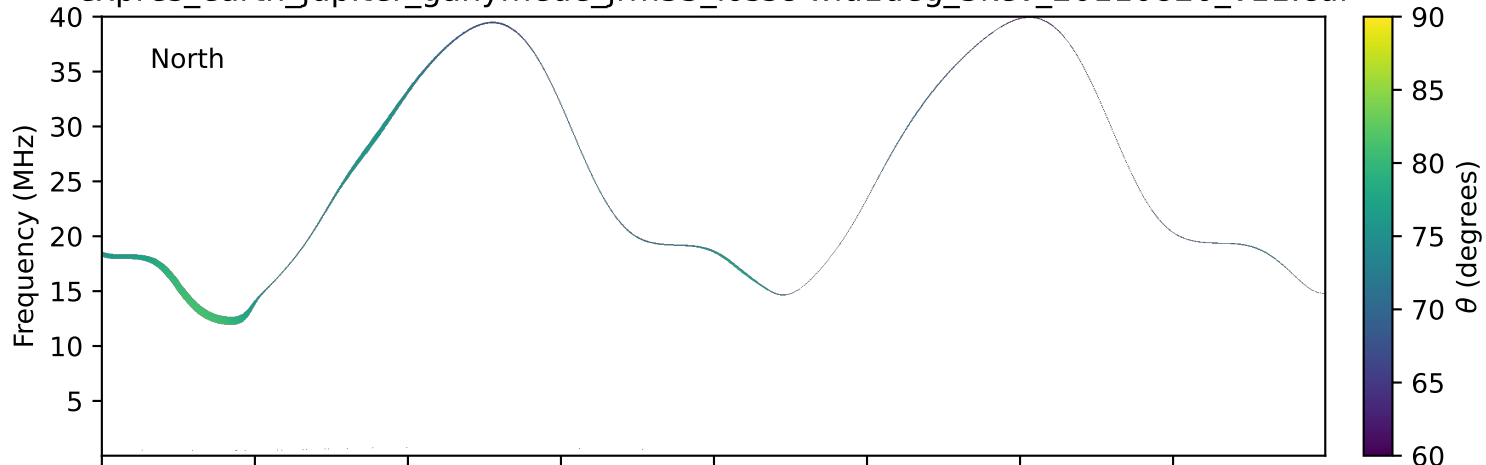
expres_earth_jupiter_ganymede_jrm33_lossc-wid1deg_3kev_20110820_v11.cdf
