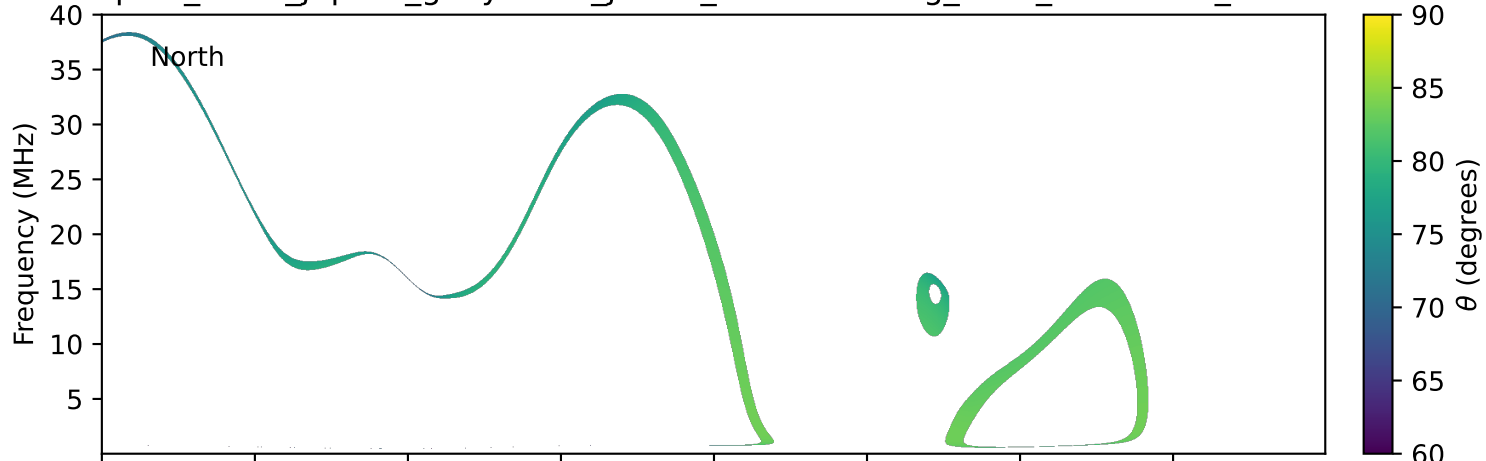
expres_earth_jupiter_ganymede_jrm33_lossc-wid1deg_3kev_20110808_v11.cdf
