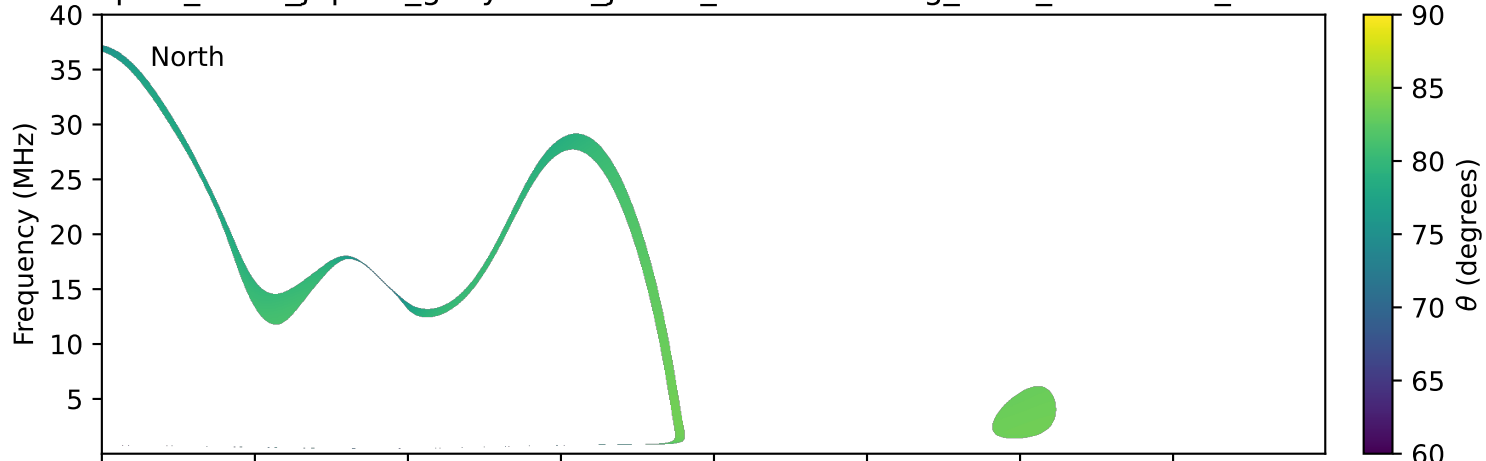
expres_earth_jupiter_ganymede_jrm33_lossc-wid1deg_3kev_20110801_v11.cdf
