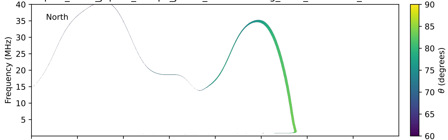
expres_earth_jupiter_europa_jrm33_lossc-wid1deg_3kev_20110826_v11.cdf
